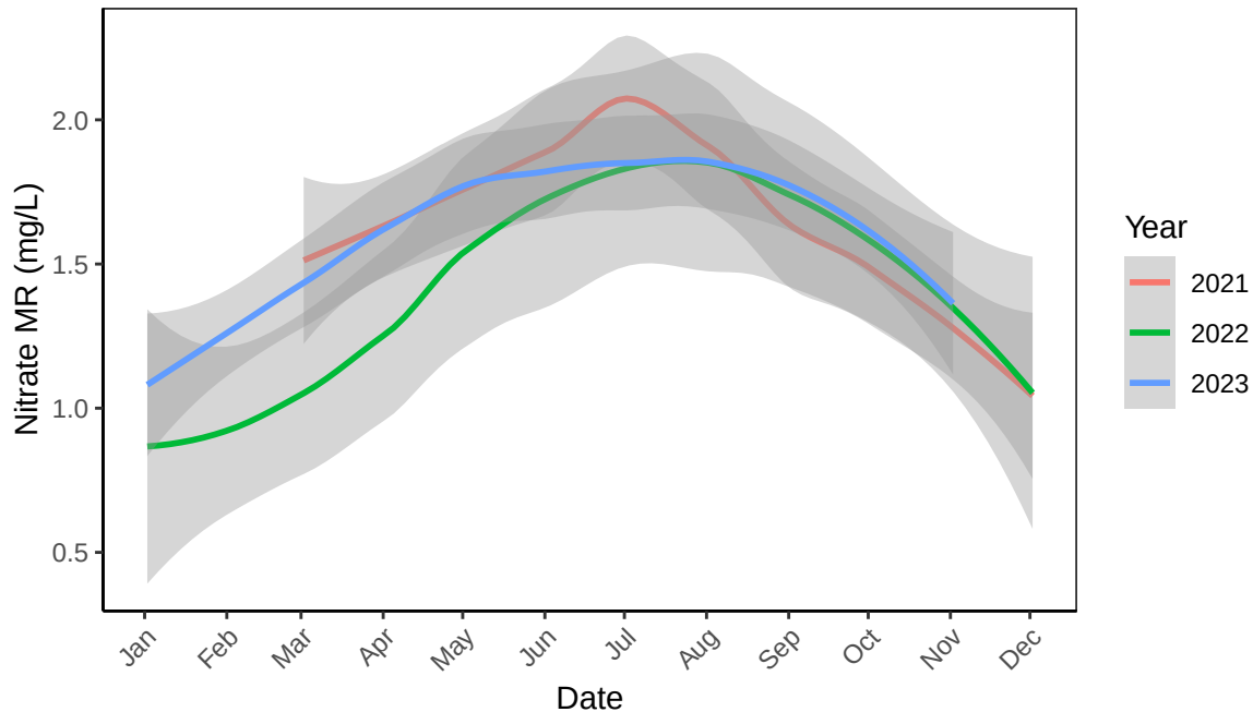
B2 Raceway 2 Nitrate MR (mg/L) Monthly Mean
